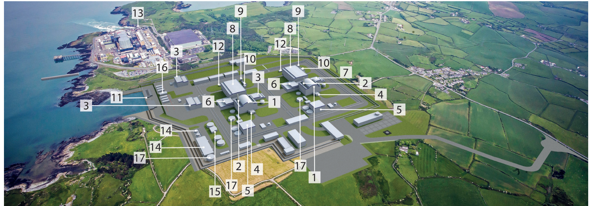
Figure 3-2 Indicative site layout – Stage One Pre-Application Consultation
